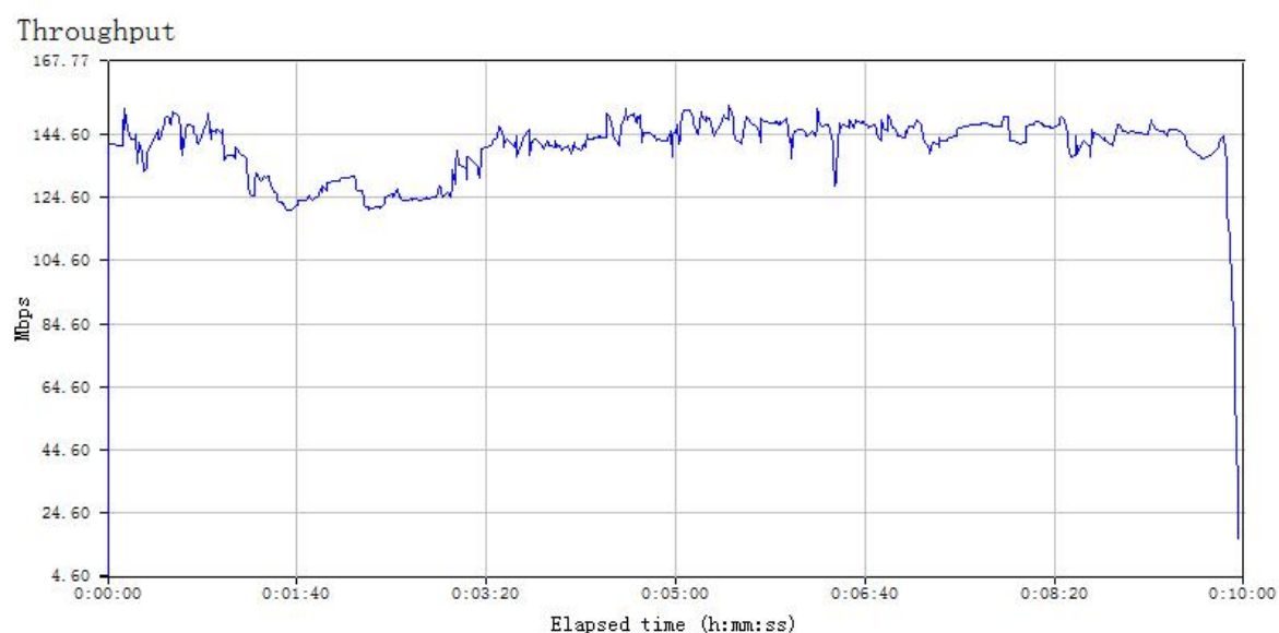
5G (AC/A/N) Throughput Test Fluctuation Chart:
