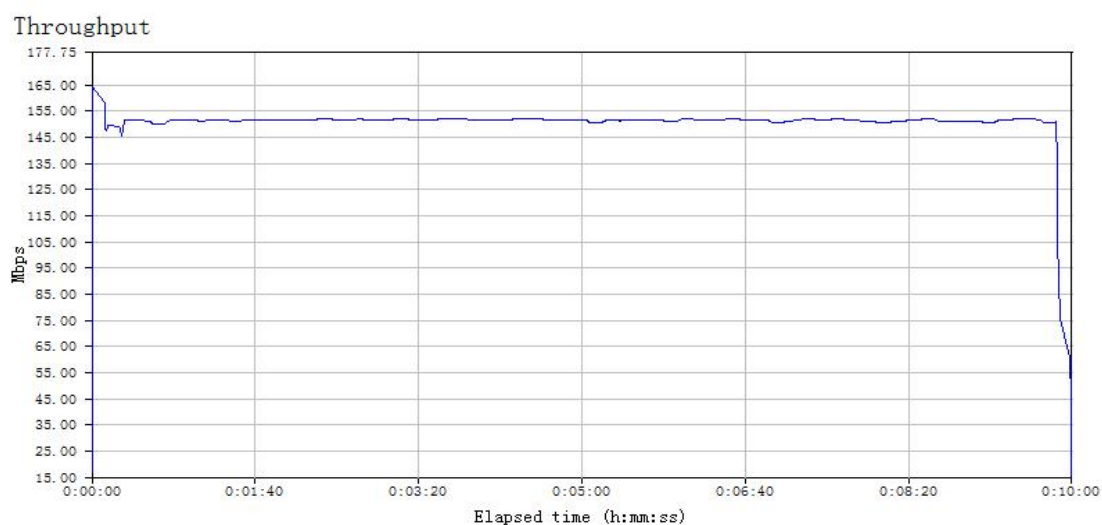
5G (AC/A/N) Throughput Test Fluctuation Chart:
